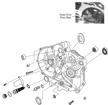
PLATE NO. : 11 CRANKCASE LH
