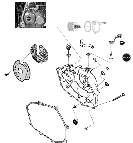
PLATE NO. : 12 COVER RH
