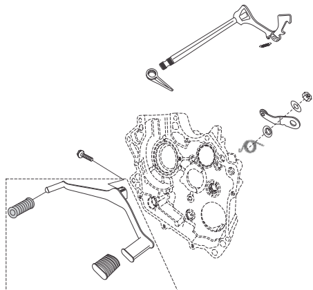
PLATE NO. : 9 GEAR CHANGE MECHANISM
