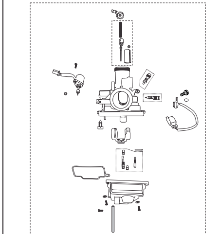
PLATE NO. : 16 CARBURETOR
