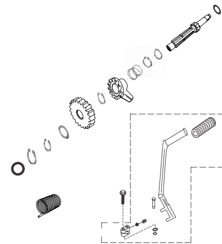
PLATE NO. : 15 KICK STARTER MECHANISM
