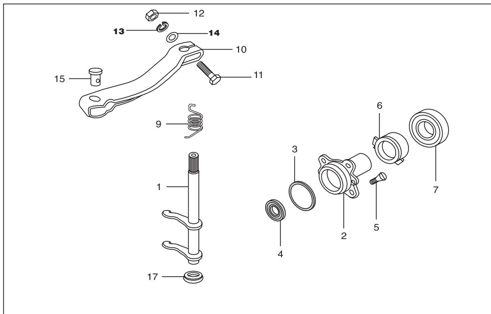
Plate No. 14 : CLUTCH SHAFT ASSEMBLY
