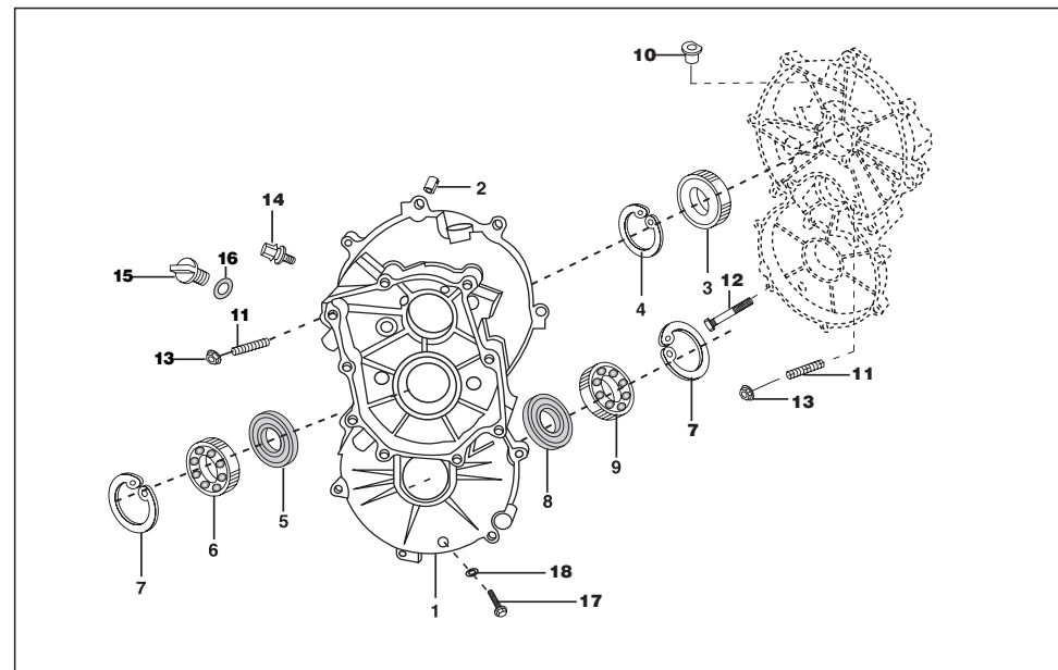
Plate No. 15 : MAIN HOUSING
