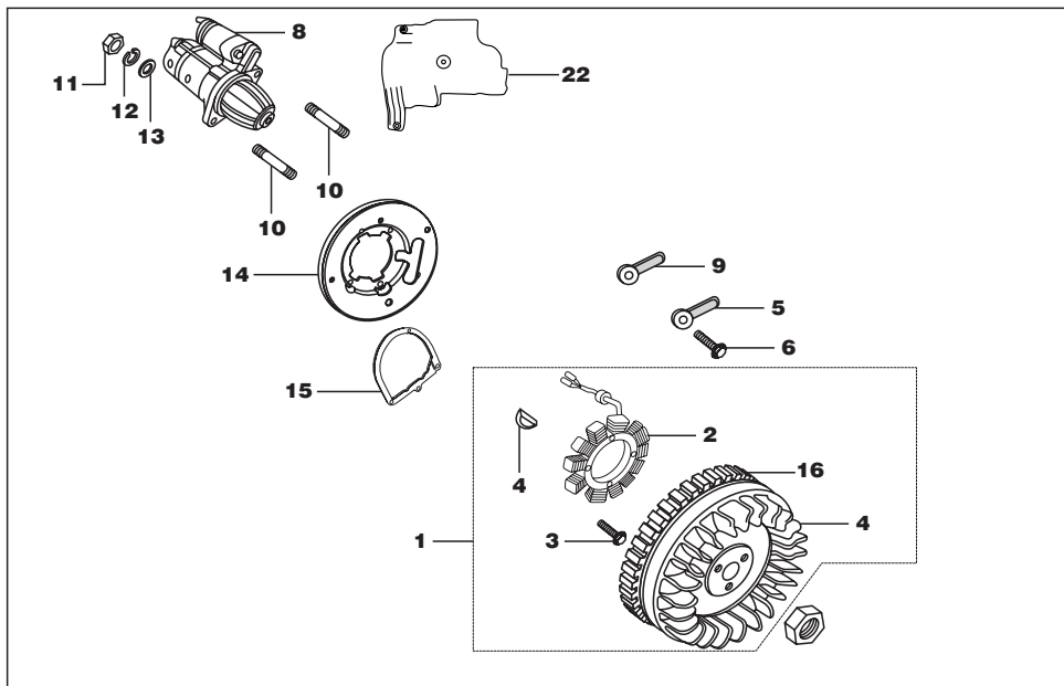
Plate No. 21 : ALTERNATOR & STARTER MOTOR | GC MAX, MEGA MAX RE 445 L DIESEL
