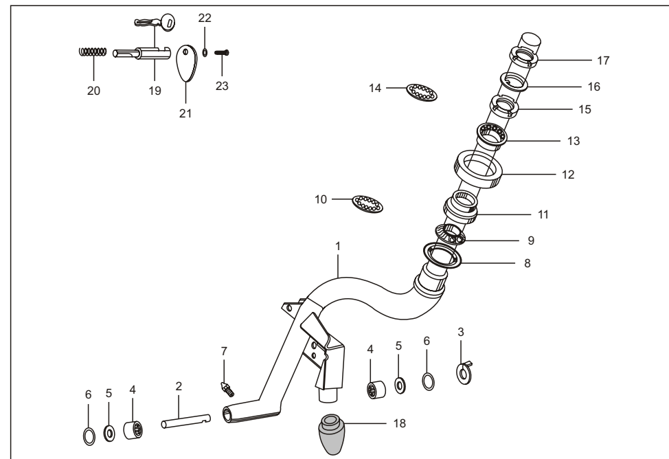
Plate No. 36 : STEERING COLUMN ASSLY
