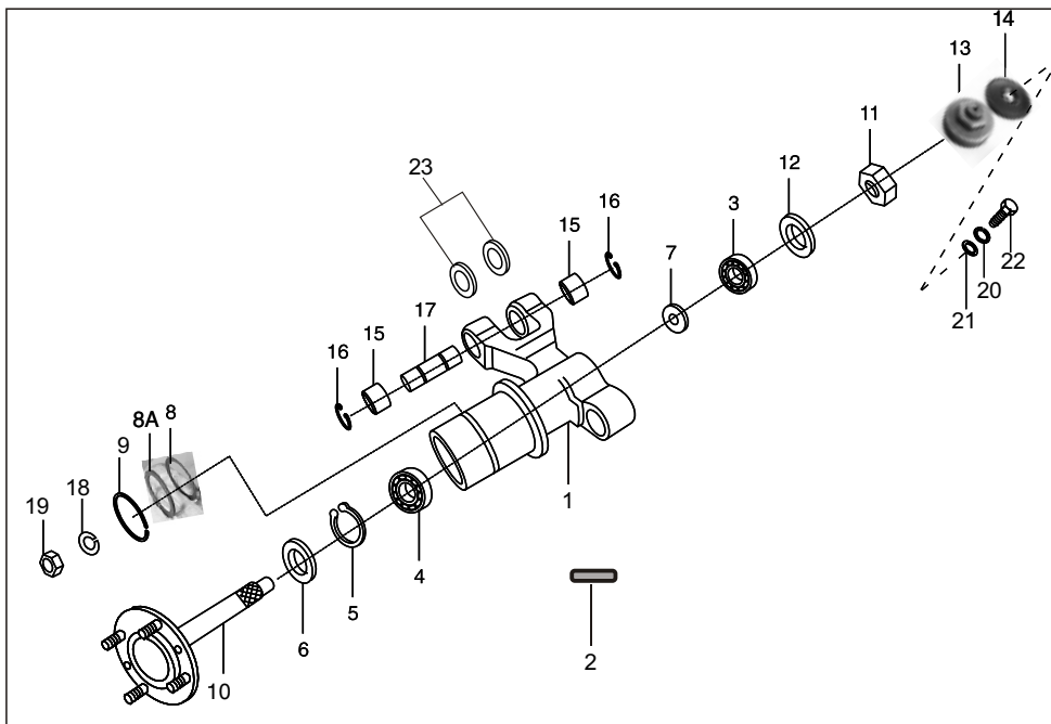
Plate No. 35a : FRONT HUB
